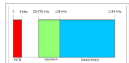
Frequency plan for ADSL. The red area is the frequency range used by normal voice telephony (PSTN), the green (upstream) and blue (downstream) areas are used for ADSL.
